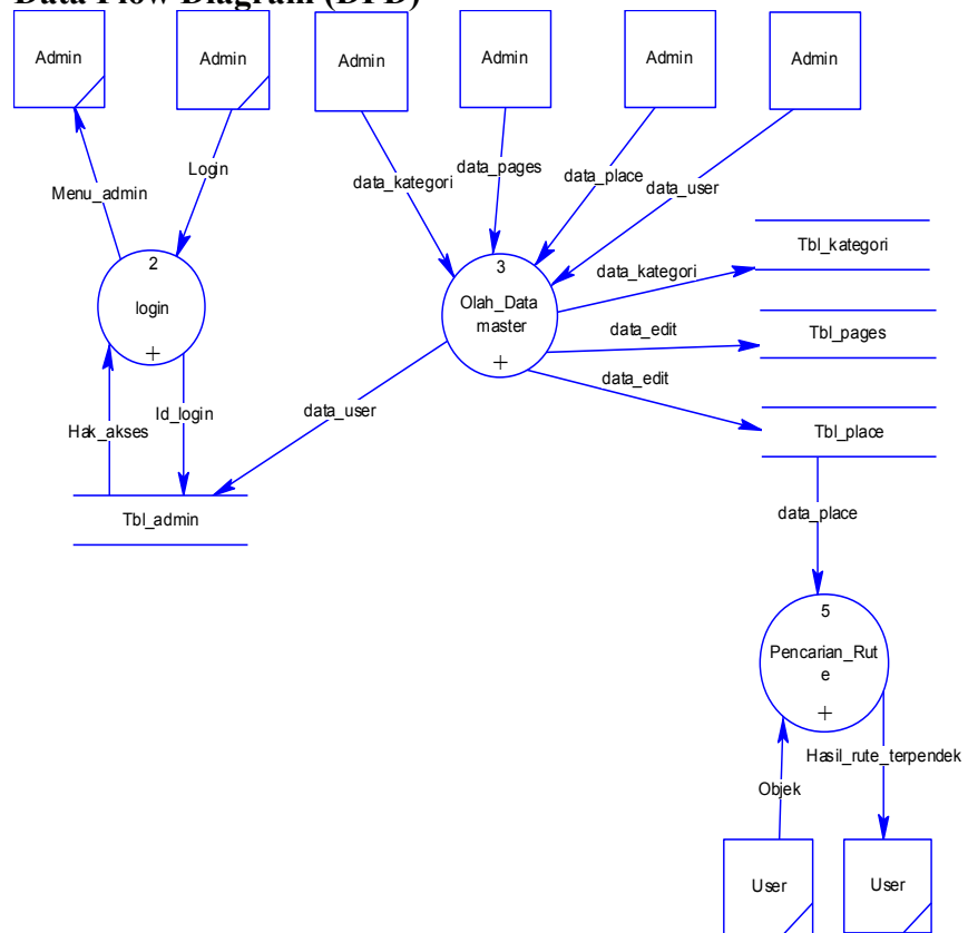
Gambar 4.3 DFD Level 1
