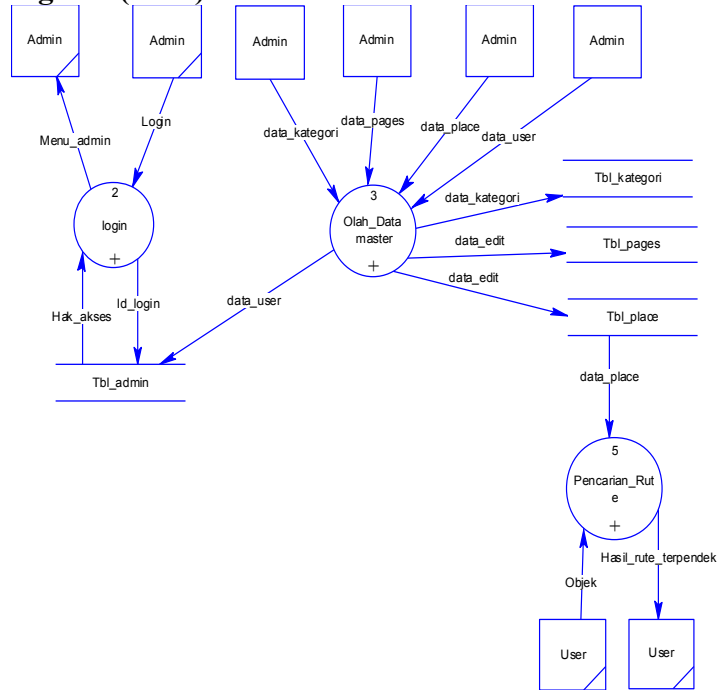
Gambar 4.3 DFD Level 1
