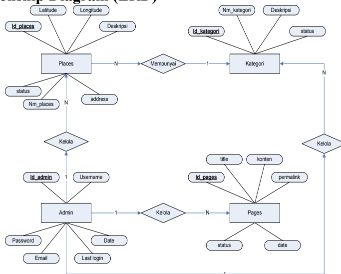
Gambar 4.6 Entity Relationship Diagram
