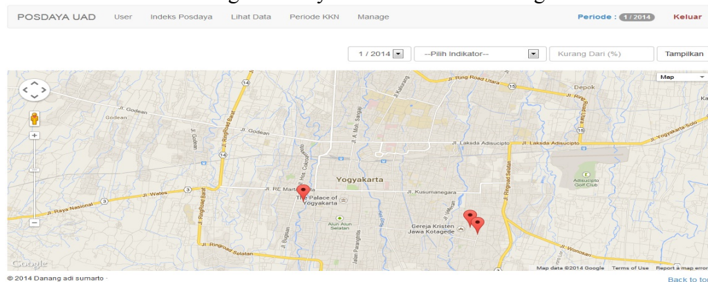
Gambar 5. Halaman Monitoring
