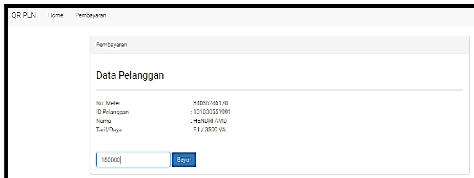
Figure 15. Payment Form
