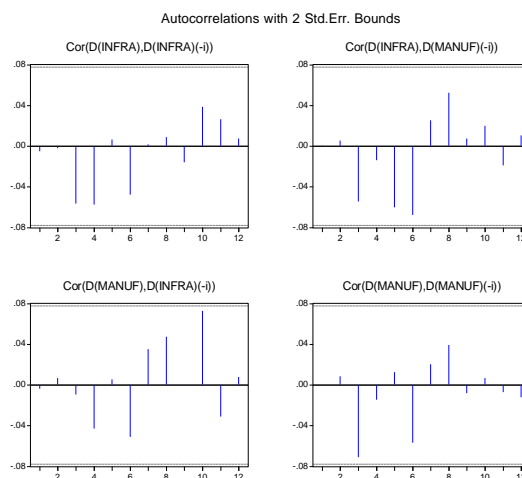
Gambar 6. Plot ACF residual model VAR(2)
