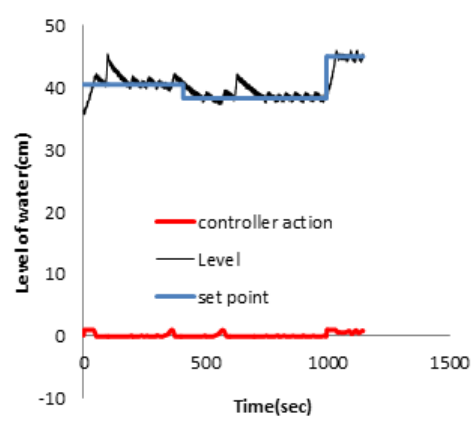
Figure 3(h). SIMC tuned MMPI Controller's Regulatory Response for region 36-45cm
