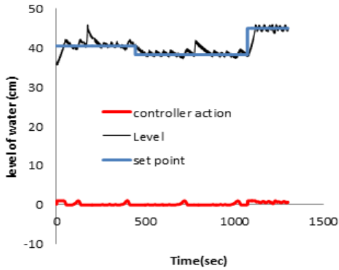
Figure 3(i). CHR tuned MMPI controller's Regulatory Response for region 36-45cm
