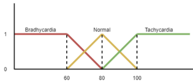
Fig. 4. Membership of Heart Rate
