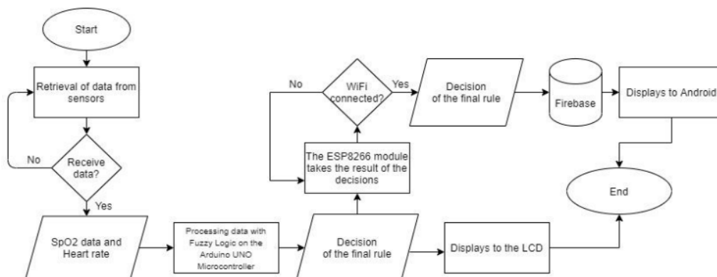
Fig. 2. System Flowchart
