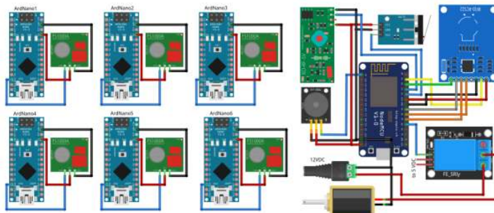
Fig 3. Inventory system electronic circuit
