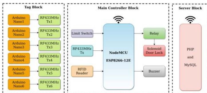
Fig 2. Inventory system block diagram
